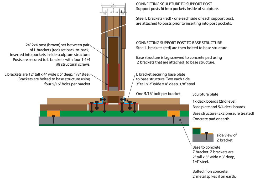
CONNECTING SCULPTURE TO BASE STRUCTURE END VIEW
