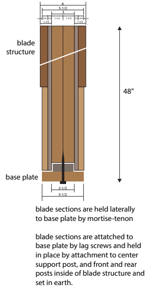
POSITIONING BLADES (LATERALLY) ON BASE PLATE END VIEW
